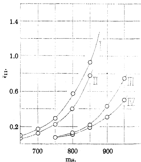
Fig. 7.—Dependence of the formal extinction coefficient of iron(II), \bar{\epsilon}_{II} , on hydrochloric acid concentration: I 4.1 F HCl, 0.31 F FeCl 2 ; II, 5.0 F HCl, 1.42 F FeCl 2 ; III, 10.4 F HCl, 0.29 F FeCl 2 ; IV, 12 F HCl, 0.08 F FeCl 2 .
