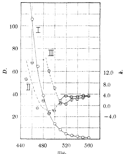
Fig. 3.—Optical interaction in the 460–560 m\mu range: I, optical density, D (referred to a 1.00 cm. light path), of 0.88 F FeCl_3 in 12 F HCl and containing 0.13 F MgCl_2 . II, III, values of k calculated using magnesium(II) and manganese(II) corrections, respectively. Concentrations identical with those of Fig. 1. (Curves are dashed in regions of large probable error.)
