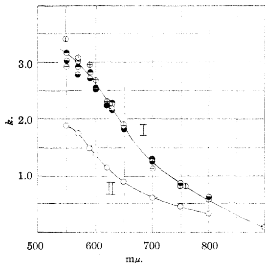
Fig. 2.—Dependence of k on wave length and hydrochloric acid concentration: I, 12 F HCl solutions. Points \odot and \ominus of this figure calculated from the data of Fig. 1, using magnesium and manganese corrections, respectively; points \circ and \bullet , solutions of Fig. 1, diluted by a factor of two, magnesium and manganese corrections, respectively. II, 5.0 F HCl solutions, data of Fig. 5 (ordinates, k \times 10 ).
